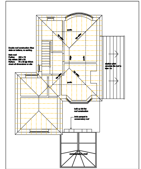
Roof plan
