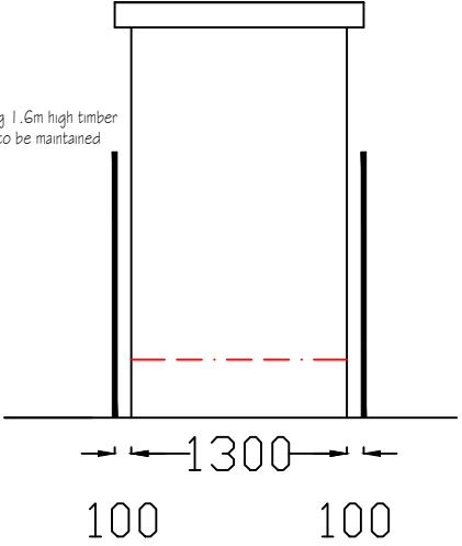
Elevation D
