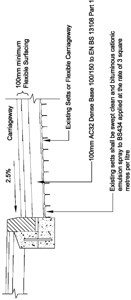
CONSTRUCTION OVER EXISTING CARRIAGEWAY
