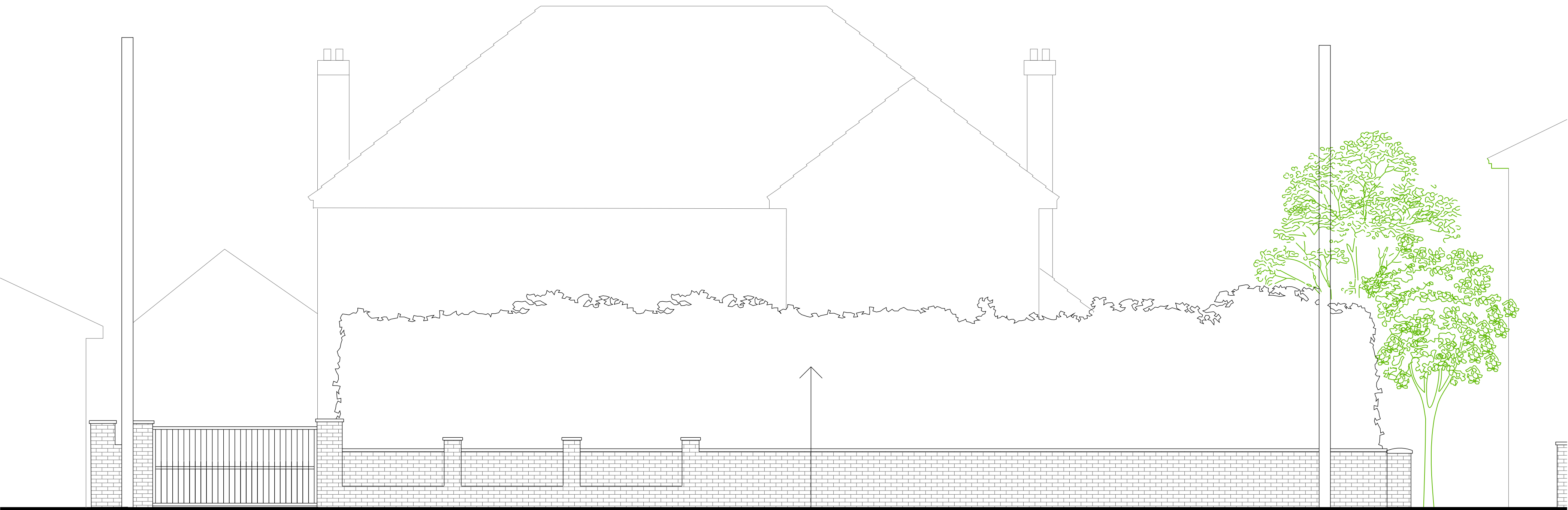
EXISTING ELEVATION
