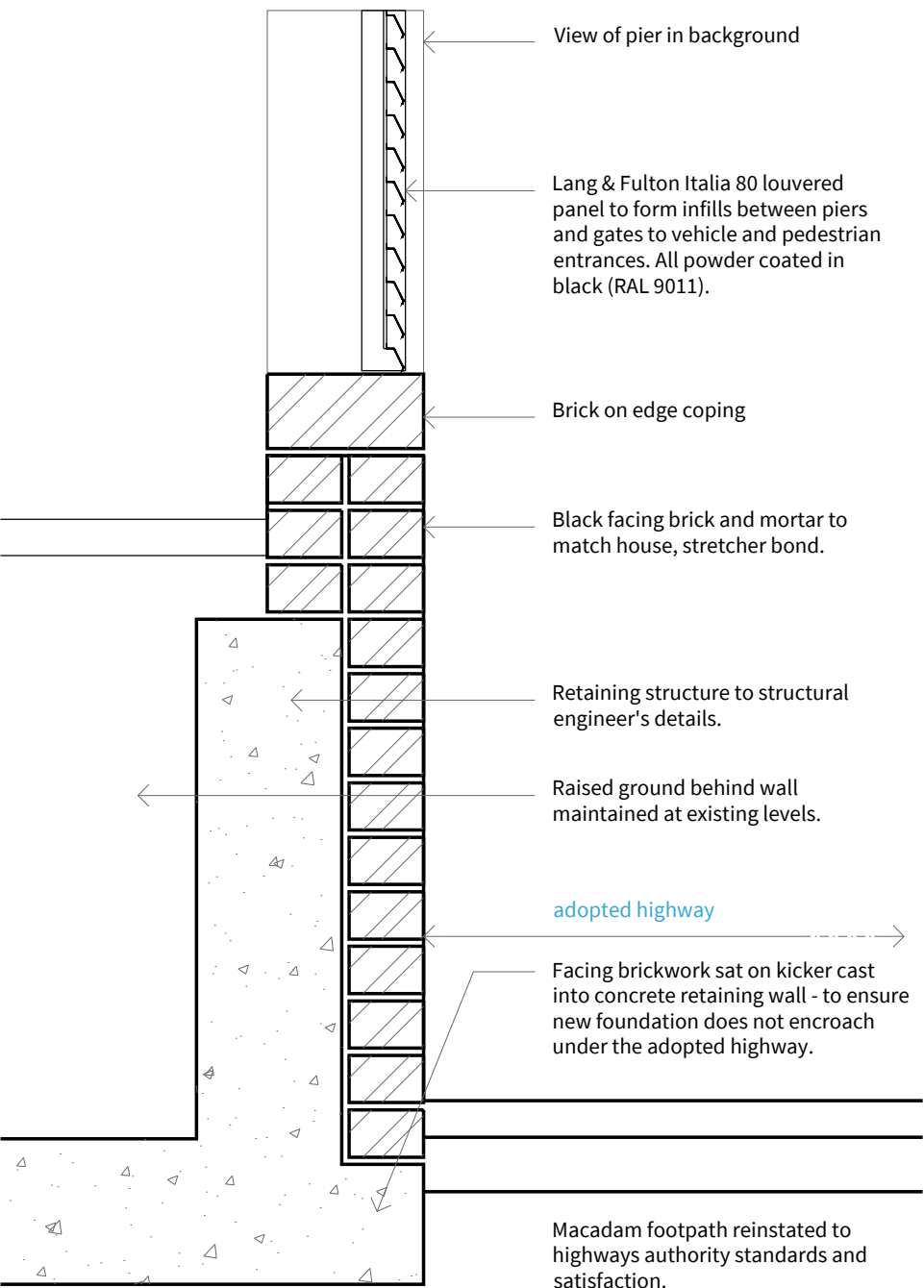
Typical section through proposed front wall. Scale 1:10
