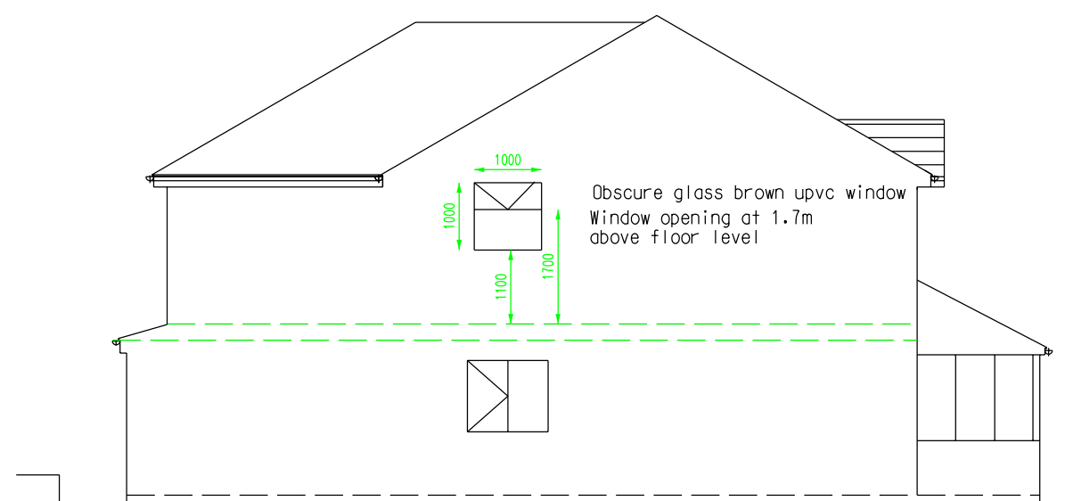
SIDE ELEVATION
