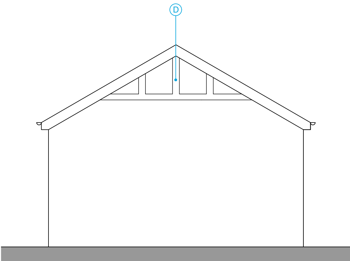
ELEVATION 03
