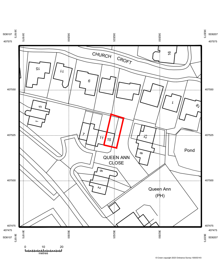
SITE LOCATION PLAN SCALE 1:1250@A4
