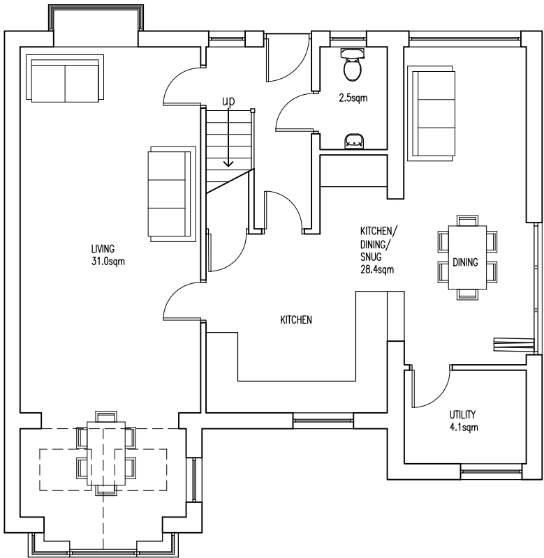
EXISTING GROUND FLOOR PLAN 1:100 @ A3
