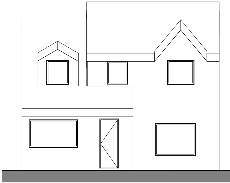
1 Proposed Elevation 1 1 : 100
