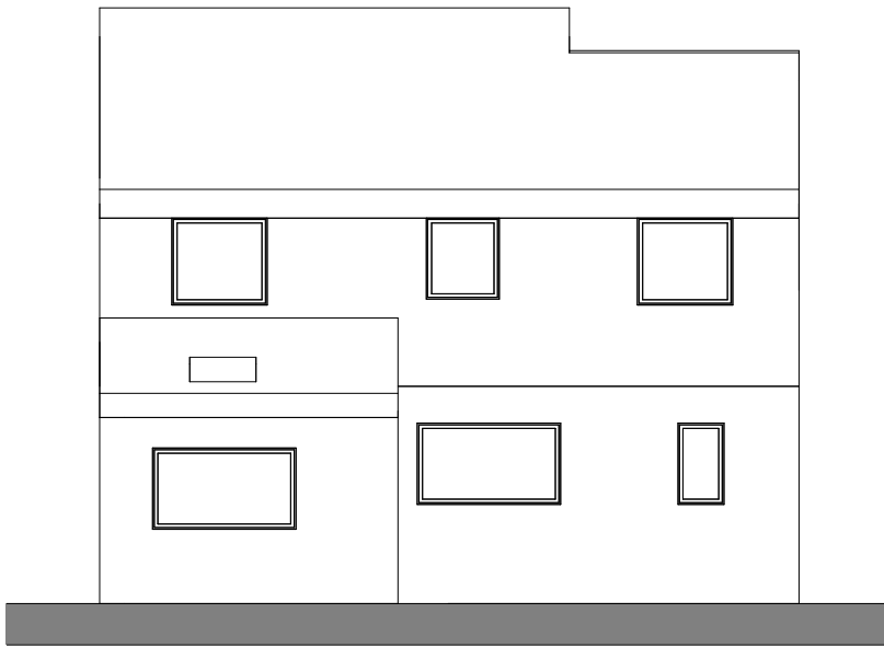
3 Proposed Elevation 3 1 : 100
