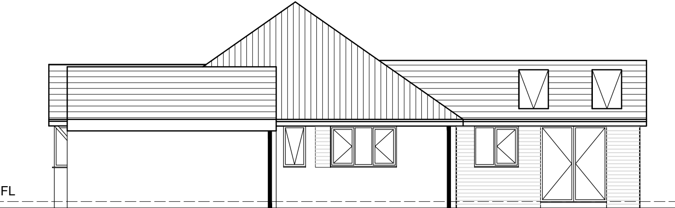
SOUTH ELEVATION 1:100
