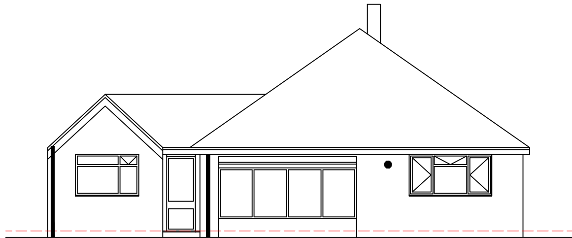
REAR ELEVATION 1:100
