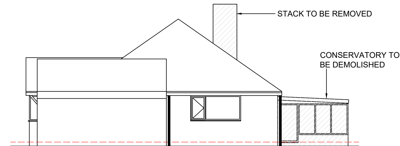
SOUTH ELEVATION 1:100
