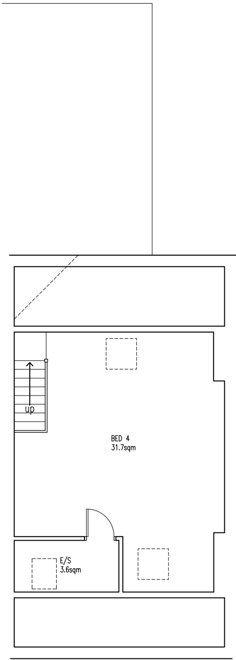
EXISTING SECOND FLOOR PLAN 1:100 @ A3
