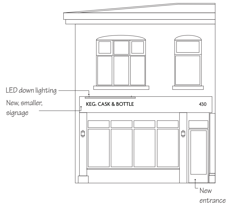
PROPOSED ELEVATION 1:100 @A4
