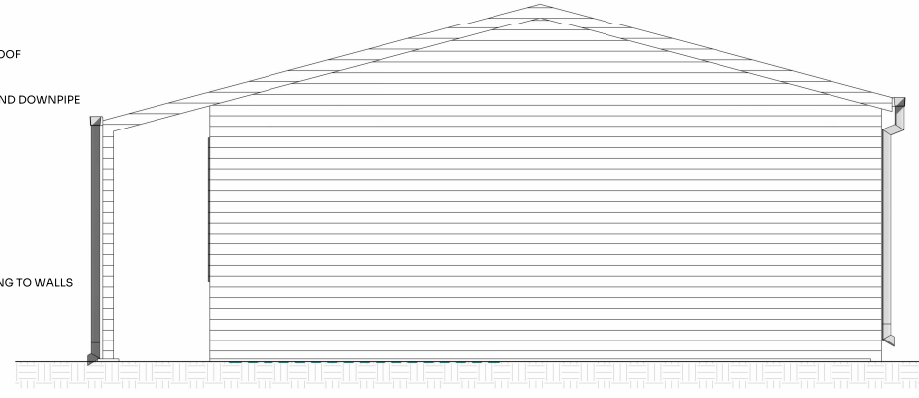
2 Classroom - East 1:25
