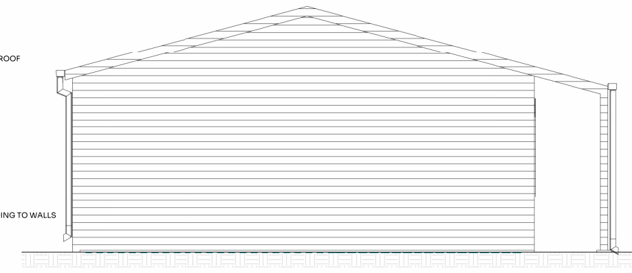
4 Classroom - West 1:25
