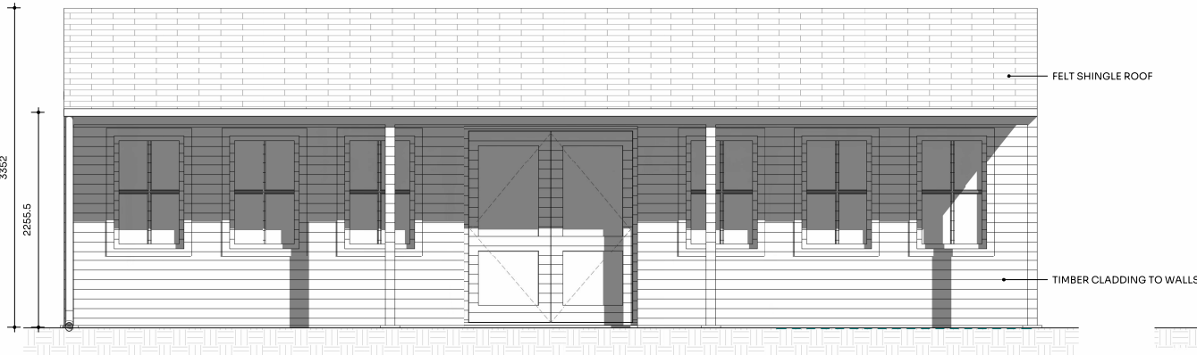
3 Classroom - South 1:25
