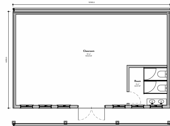
5 Classroom Plan 1:50
