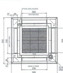
Lower View
